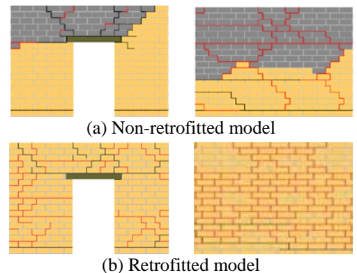
Fig. 8 East and south wall crack patterns (Cracks before Run 41: Black; Cracks after Run 41: Red)
