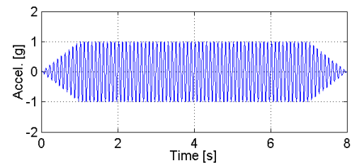
Fig. 3 Input motion waveform ( f=10\text{Hz} , A=1\text{g} )
