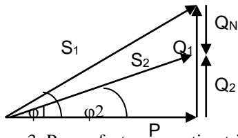
Figure 3: Power factor correction triangle
