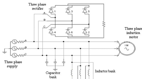
Figure 2. Electrical circuit diagram of the studied system
