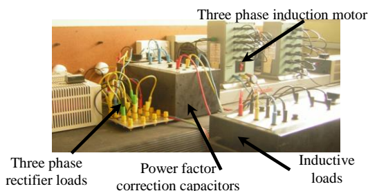
Figure 1. Photograph of the experimental setup
