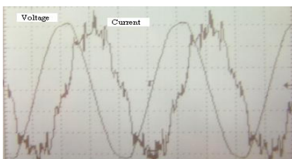
Figure 7. Waveforms of the capacitor current and harmonic load current with supply voltage
